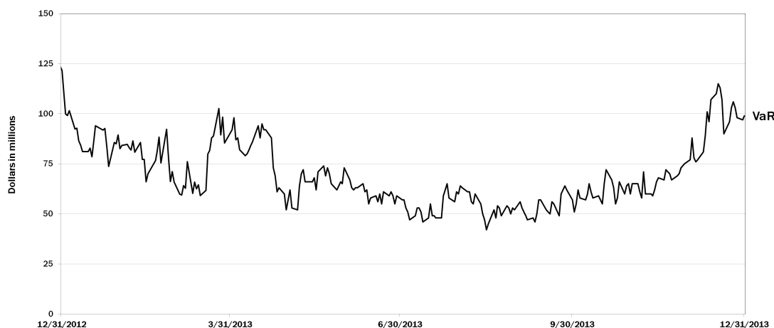
Daily Total Market-based Trading Portfolio VaR History
