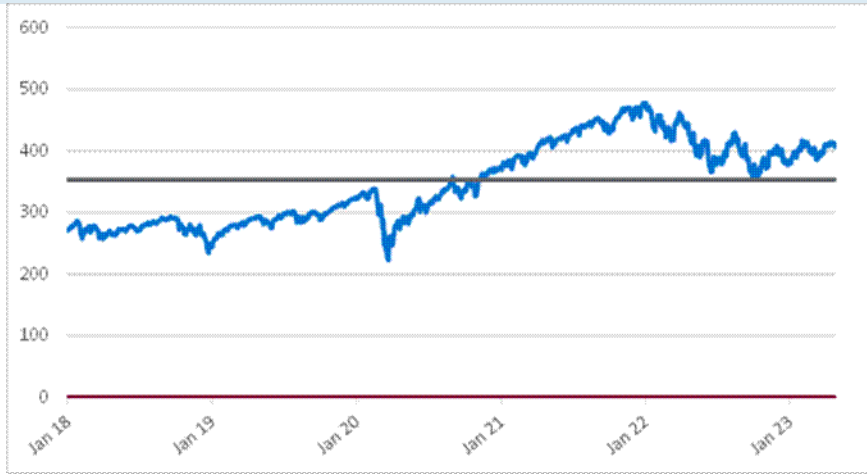
SPY Shares – Daily Closing Prices January 1, 2018 to April 25, 2023
