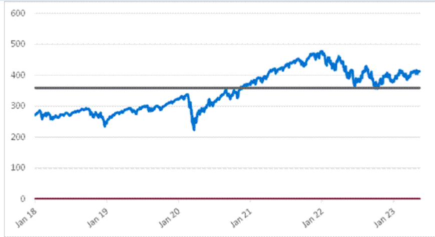
SPY Shares – Daily Closing Prices January 1, 2018 to May 15, 2023
