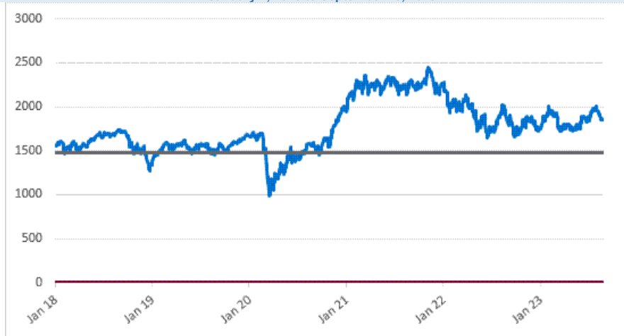
RTY Daily Closing Values January 2, 2018 to September 15, 2023
