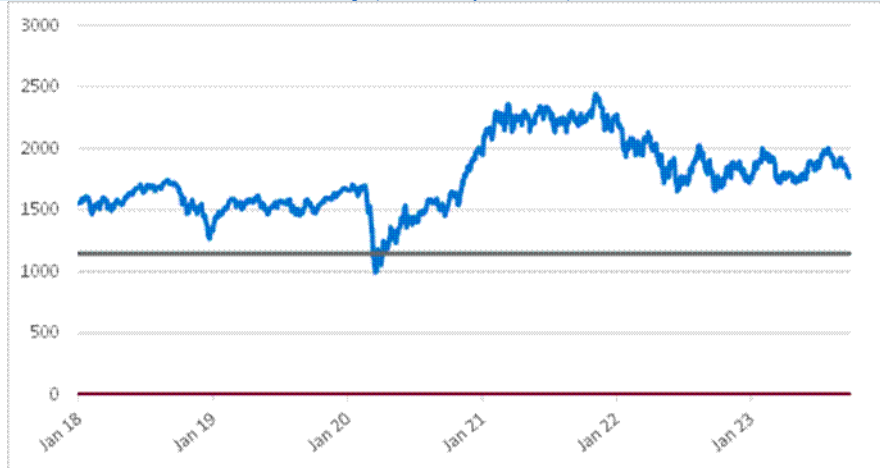
RTY Daily Closing Values January 2, 2018 to September 26, 2023
