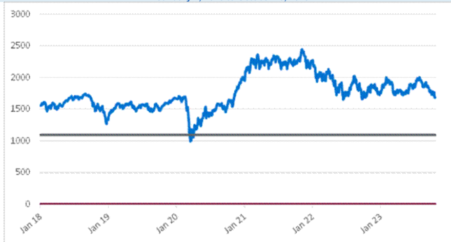
RTY Daily Closing Values January 2, 2018 to October 20, 2023
