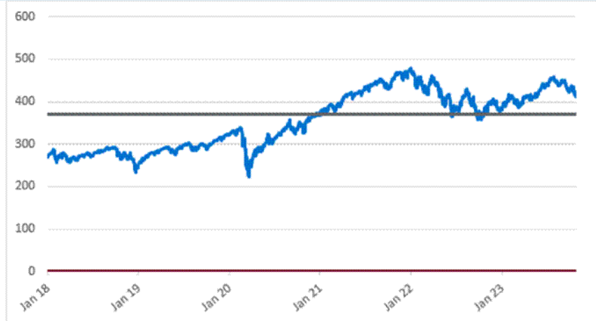
SPY Shares – Daily Closing Prices January 1, 2018 to October 26, 2023
