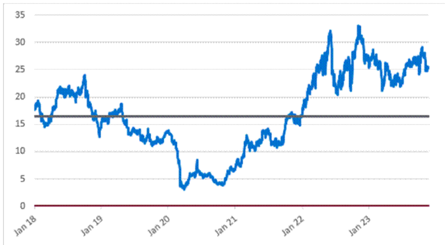
Common Stock of Marathon Oil Corporation – Daily Closing Prices January 2, 2018 to November 24, 2023
