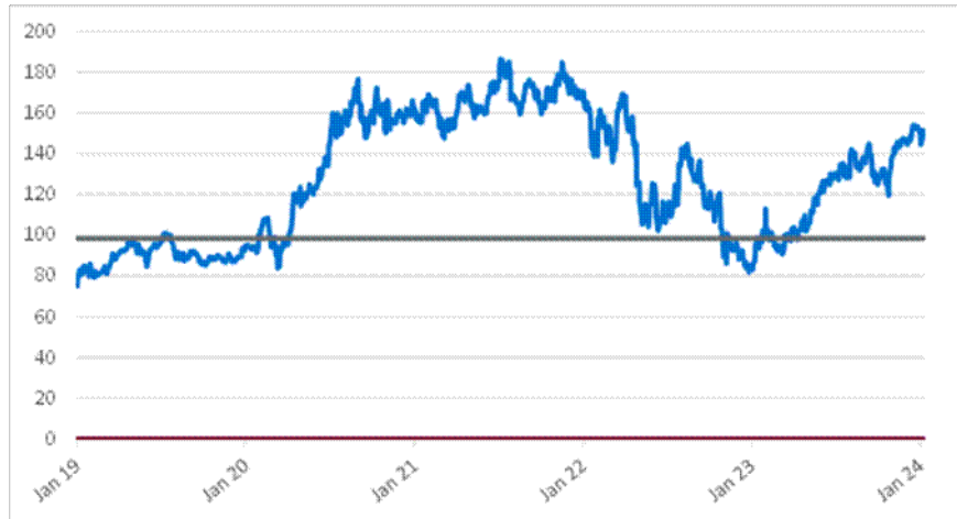
Common Stock of Amazon.com, Inc. – Daily Closing Prices January 2, 2019 to January 9, 2024
