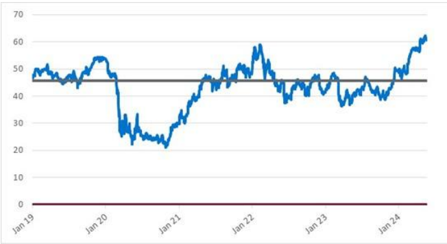
Common Stock of Wells Fargo & Company – Daily Closing Prices January 2, 2019 to May 22, 2024
