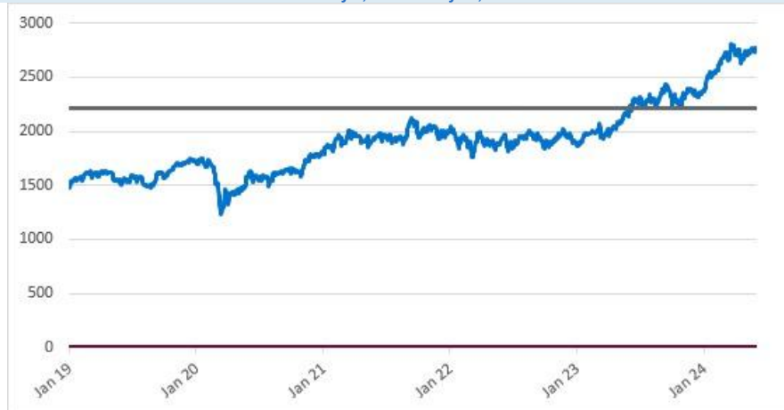
TPX Daily Closing Values January 2, 2019 to May 31, 2024
