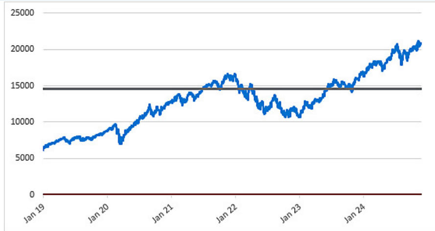
NDX Daily Closing Values January 2, 2019 to November 25, 2024
