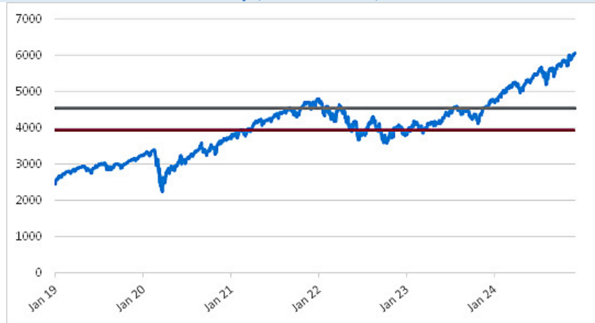
SPX Daily Closing Values January 2, 2019 to December 3, 2024
