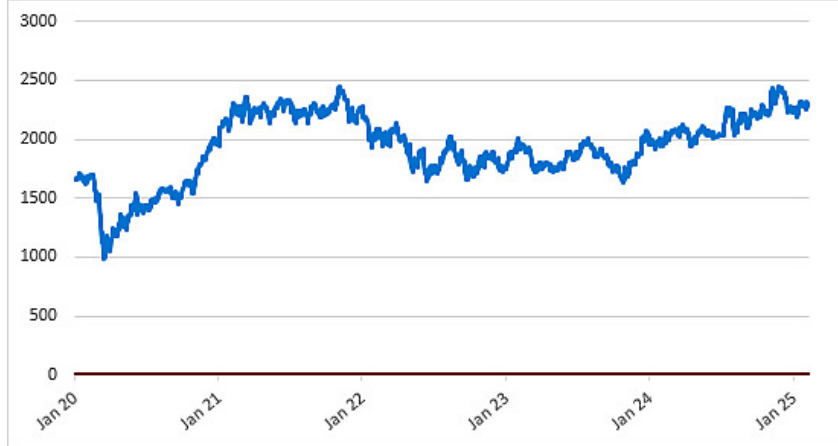
RTY Daily Index Closing Values January 2, 2020 to February 10, 2025
