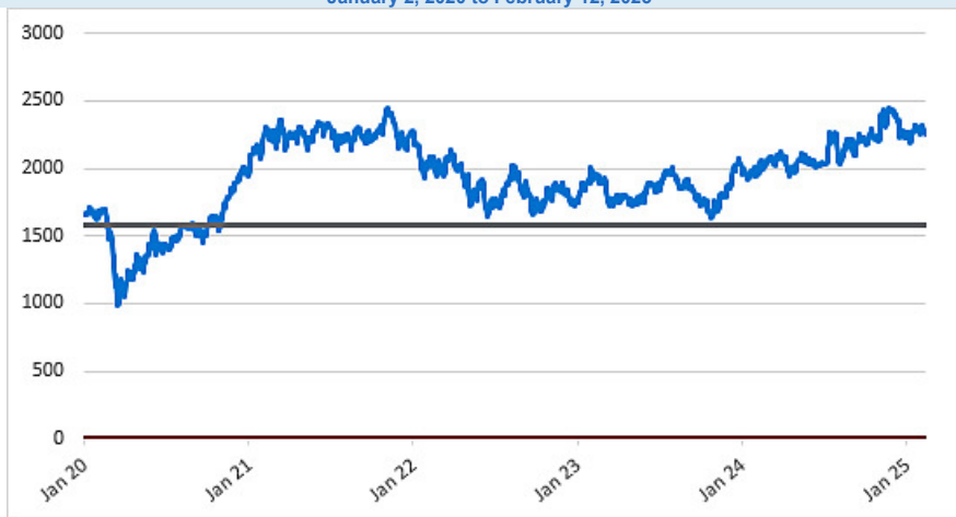
RTY Daily Closing Values January 2, 2020 to February 12, 2025
