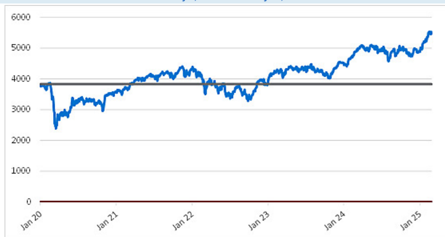
SX5E Daily Closing Values January 2, 2020 to February 28, 2025
