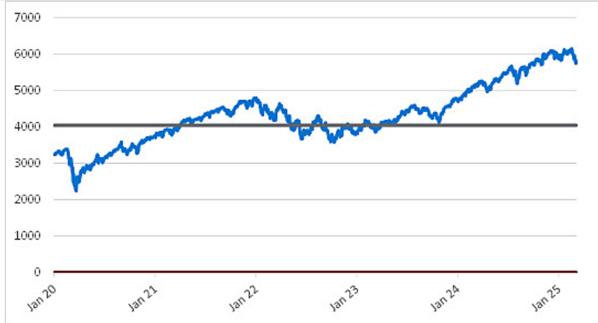
SPX Daily Closing Values January 2, 2020 to March 7, 2025
