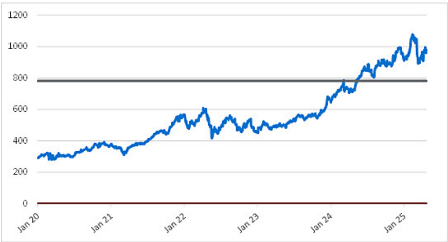
Common Stock of Costco Wholesale Corporation – Daily Closing Prices January 2, 2020 to April 23, 2025
