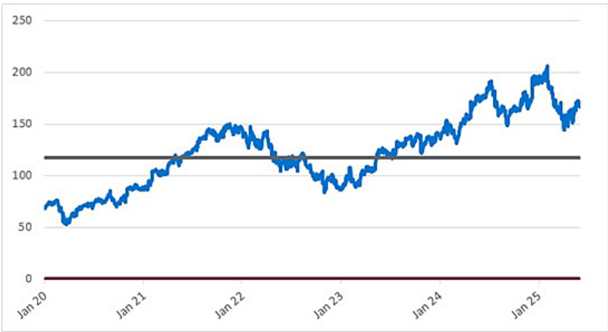
Class A Common Stock of Alphabet Inc. – Daily Closing Prices January 2, 2020 to June 4, 2025
